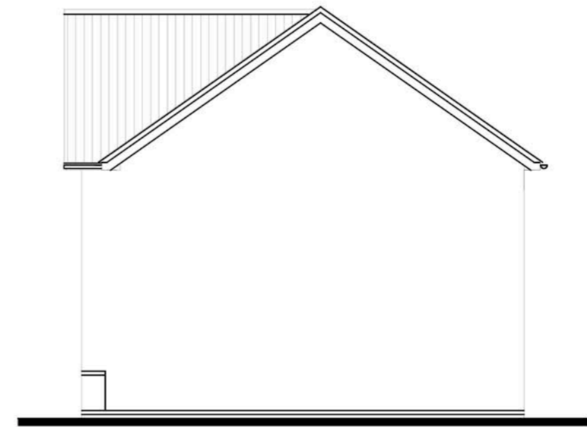
SIDE ELEVATION Radleigh
