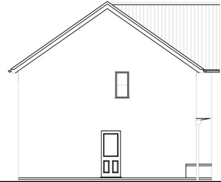
SIDE ELEVATION Radleigh
