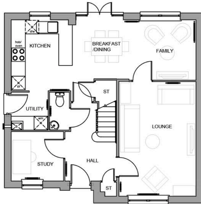
GROUND FLOOR PLAN Radleigh
